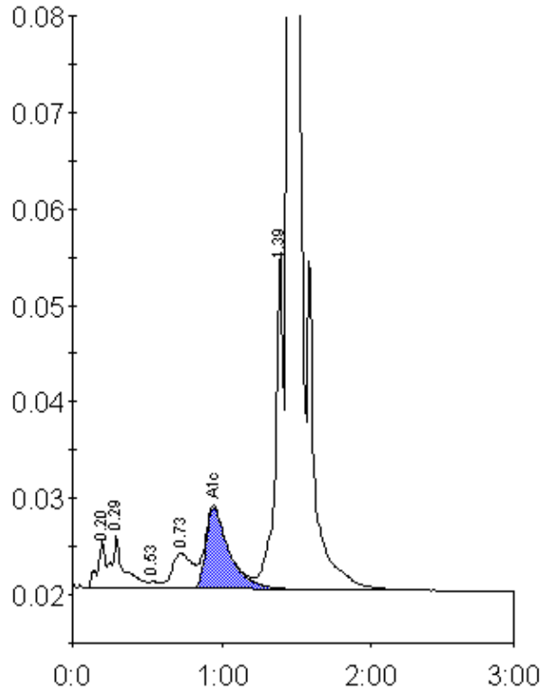
Peak table - ID: 10514117
